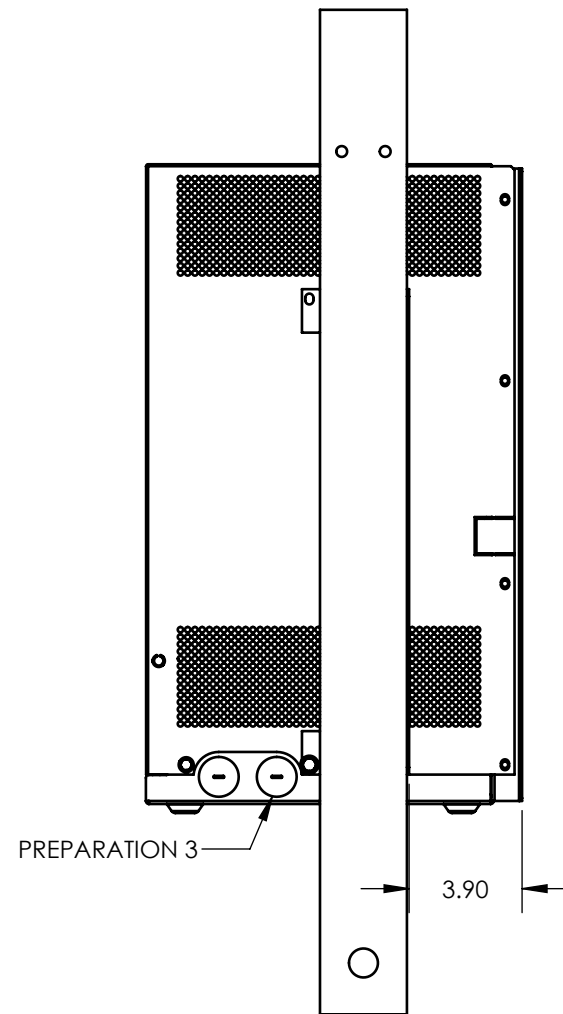
RIGHT SIDE
