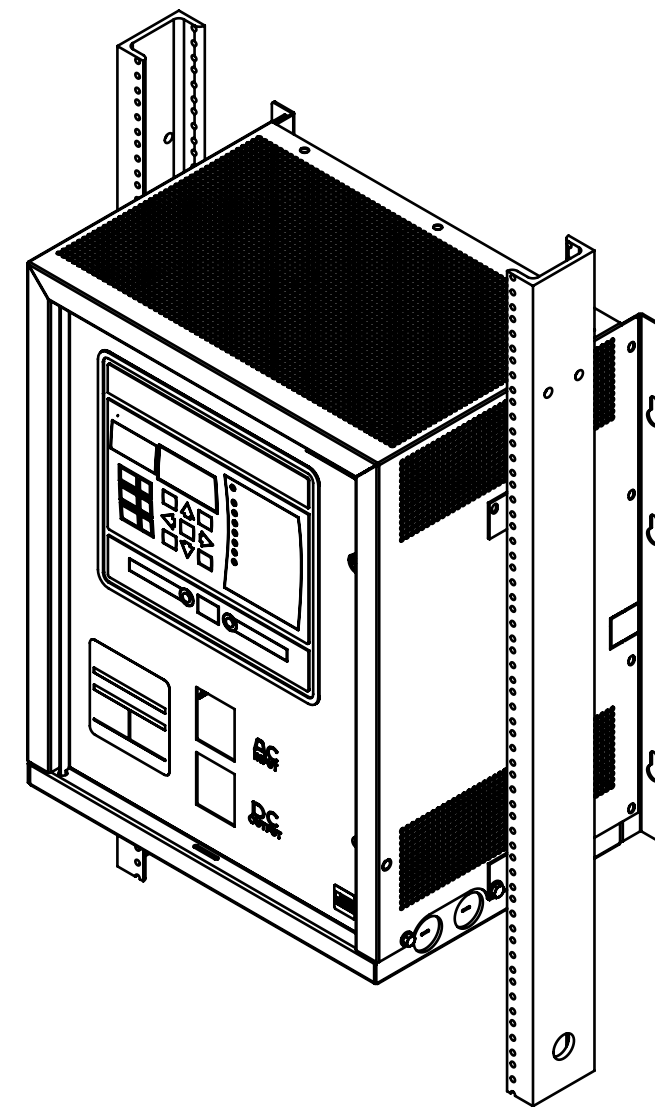
ISO VIEW
