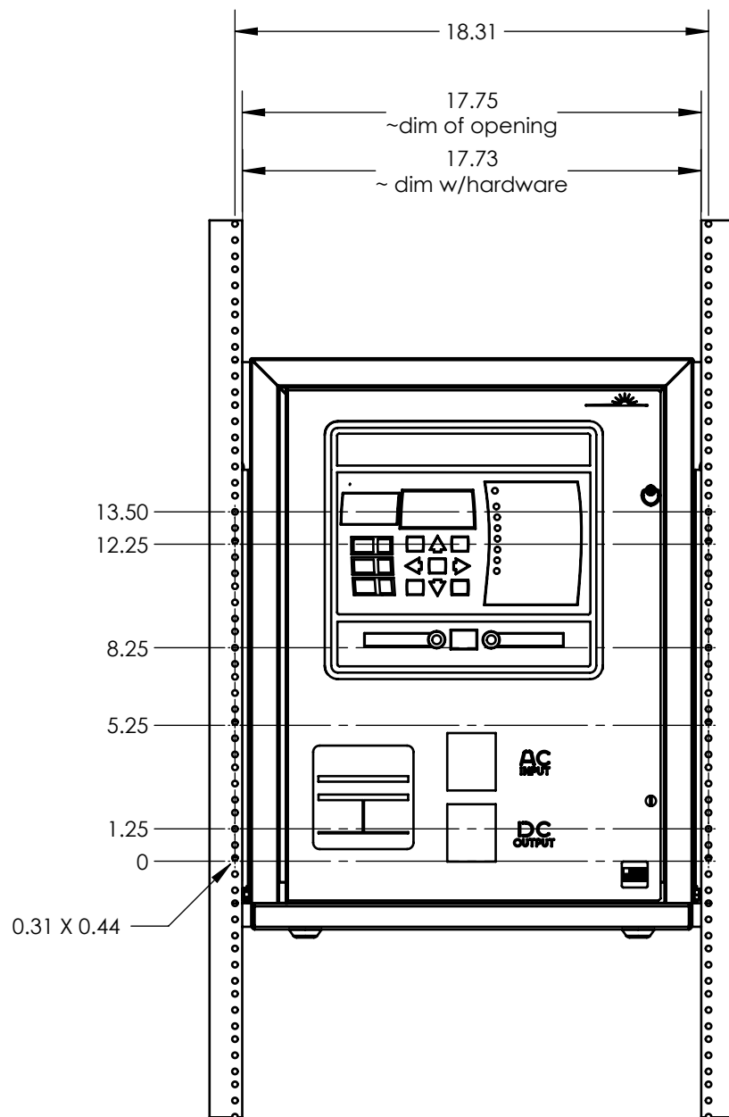
FRONT VIEW
