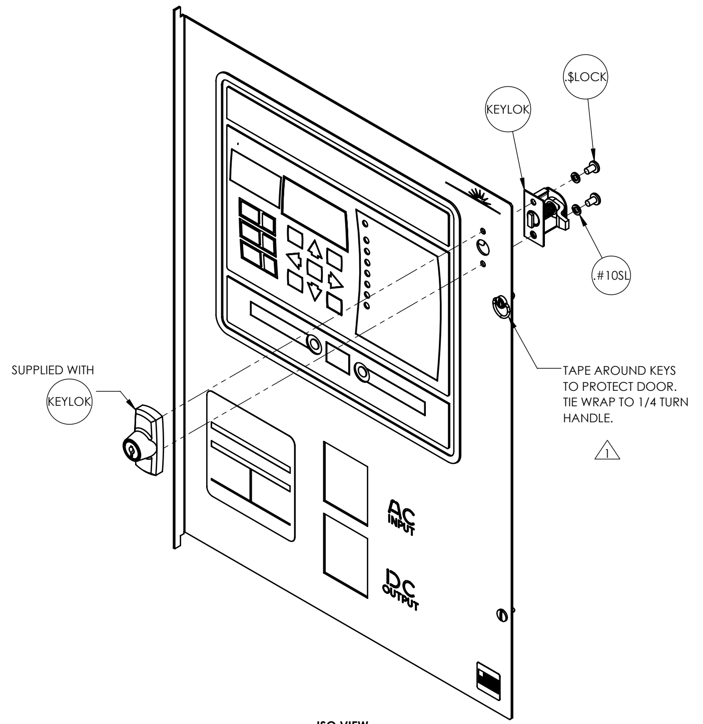
ISO VIEW DOOR ASSY
