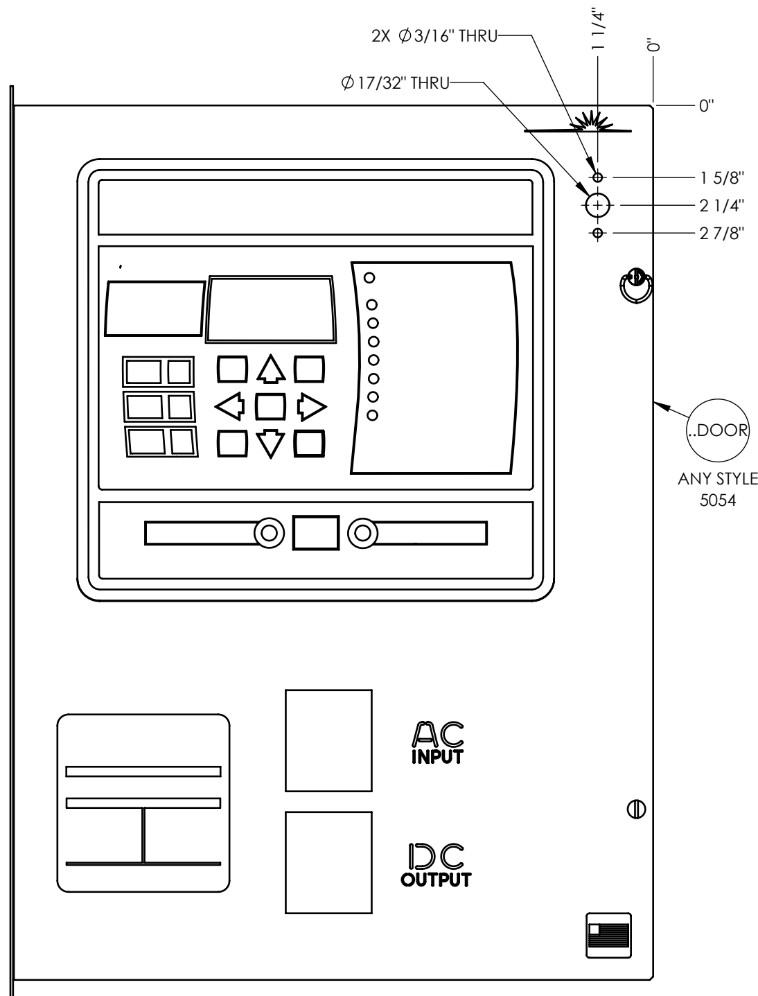
FRONT VIEW DOOR MOD
