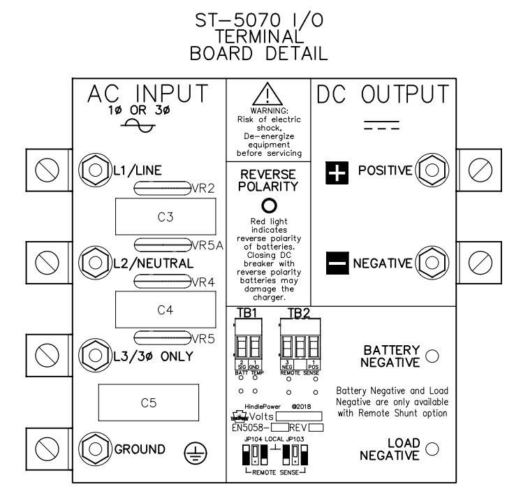
MOV PC BOARD (A9)
