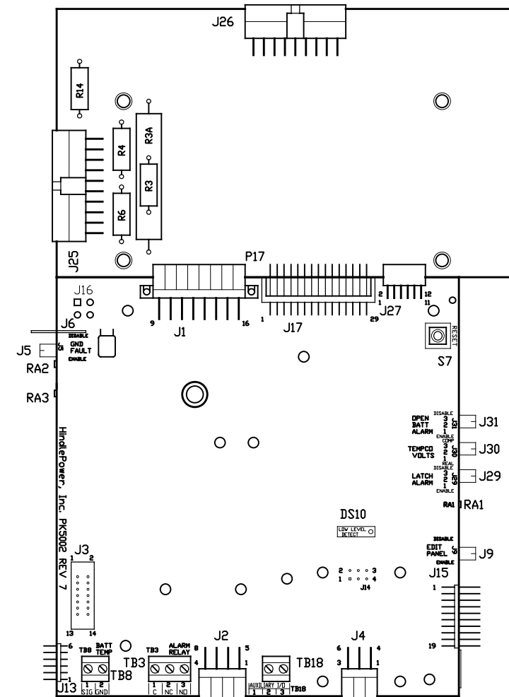
MAIN CONTROL PC BOARD (A1)
